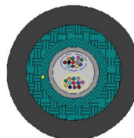
Universal Unitube up to 24 fibres
