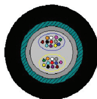
Universal Central Loose Tube
